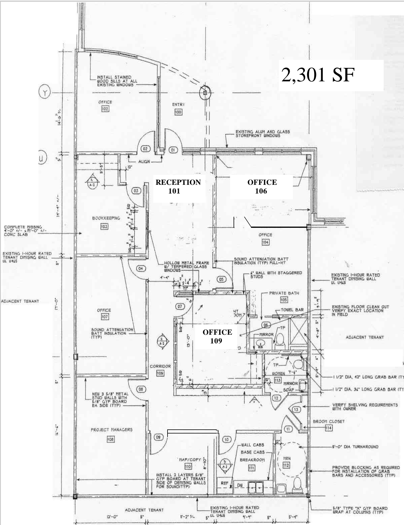
1 FLOOR PLAN A-1 1/4" = 1'-0"
