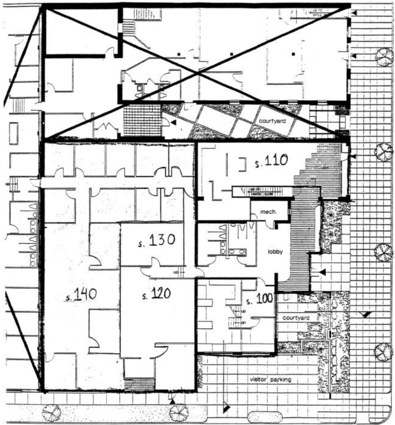
30feet 20 10 5 0 FLOOR PLAN / SITE PLAN north
